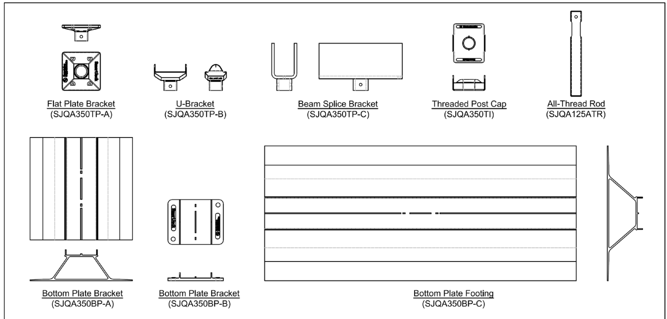
FIGURE 1 – SmartJack System Assemblies and Components
