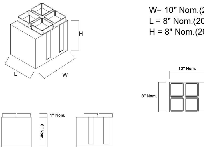
FIGURE 5 – RENCo Ledger Block
