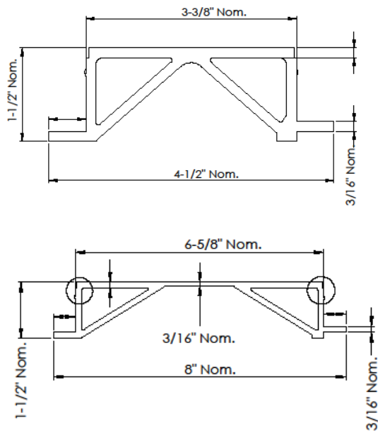
FIGURE 1 – Decking Standard Units
