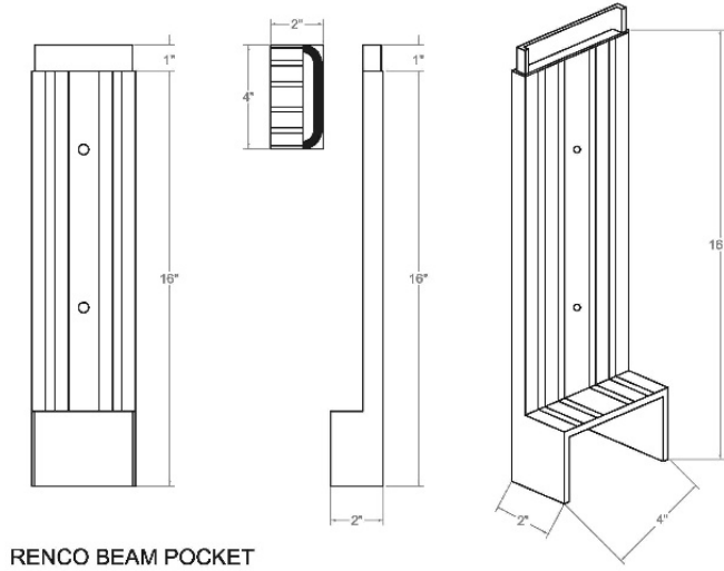
FIGURE 4 – Beam Pocket
