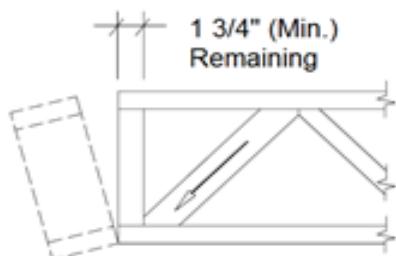
FIGURE 1 - ALLOWABLE TRUSS END TRIM
