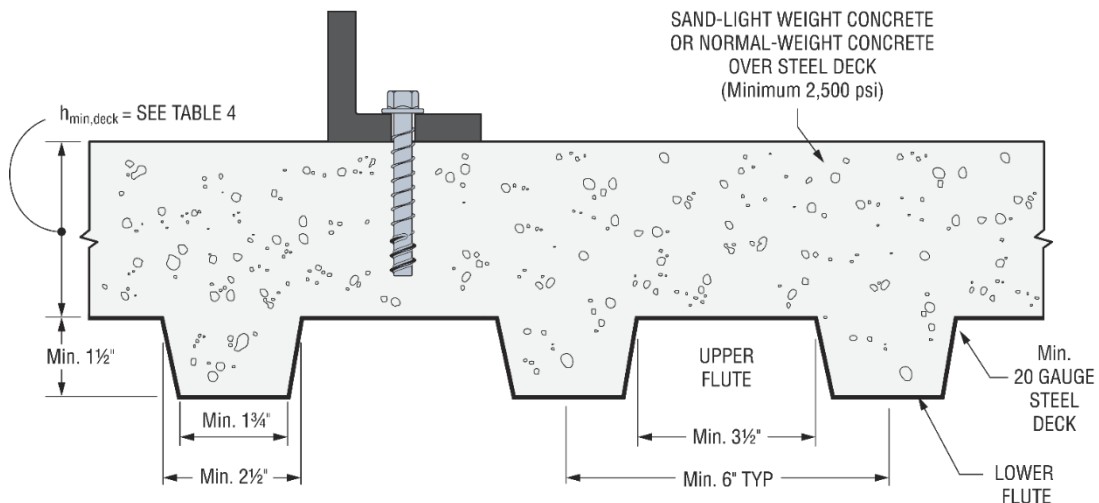
FIGURE 3 – INSTALLATION OF THE 1/4-INCH, 3/8-INCH, AND 1/2-INCH DIAMETER ANCHORS IN THE TOPSIDE OF CONCRETE-FILLED PROFILE STEEL DECK FLOOR AND ROOF ASSEMBLIES (1 in. = 25.4 mm)
