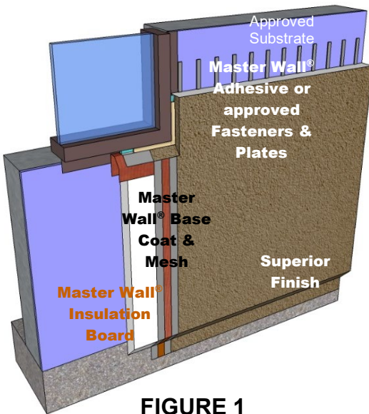
FIGURE 1 Aggre-flex EIFS
