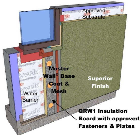
FIGURE 4 QRW1 Drainage EIFS
