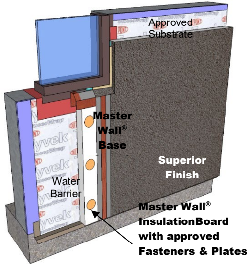
FIGURE 2 Aggre-flex Drainage EIFS
